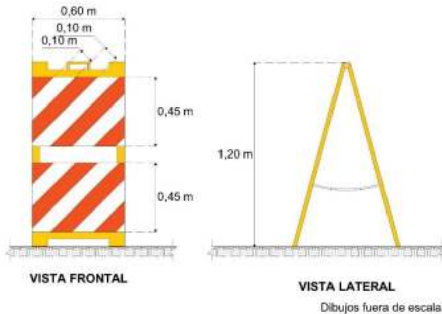
Figura V.6-3 Caballete
