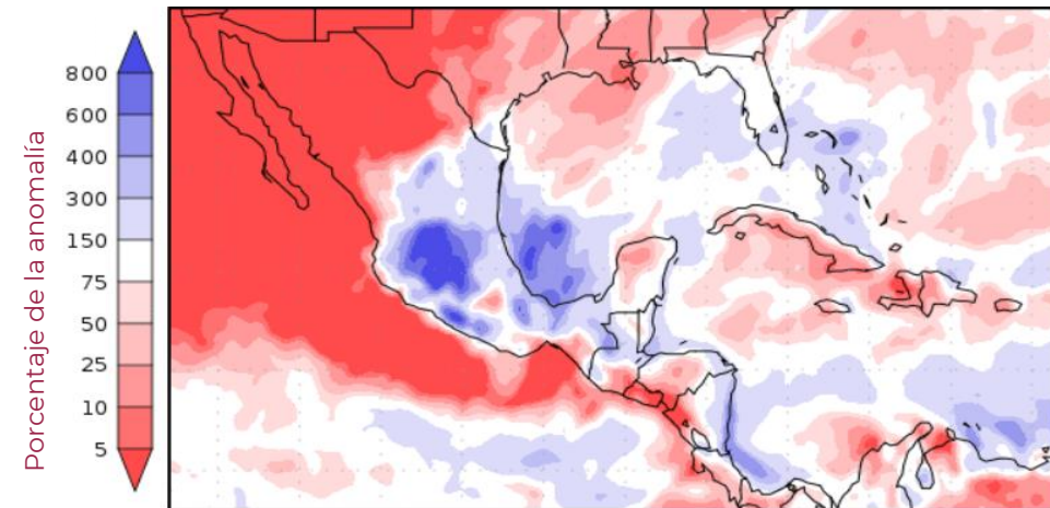
Precipitation forecasts from the National Centers for Environmental Prediction. Normal rainfall derived from Xie-Arkin (CMAP) Monthly Climatology for 1979-2003. Forecast Initialization Time: 12Z05DEC2023
