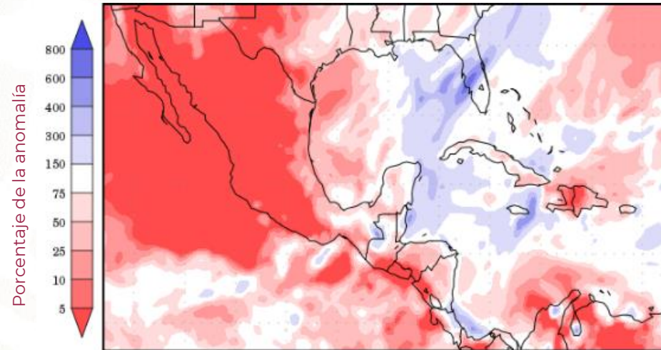
Precipitation forecasts from the National Centers for Environmental Prediction. Normal rainfall derived from Xie-Arkin (CMAP) Monthly Climatology for 1979-2003. Forecast Initialization Time: 00Z19DEC2018
